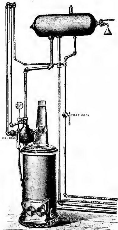
Fig. 2969. McELROY COMMINGLER SYSTEM OF CAR HEATING
